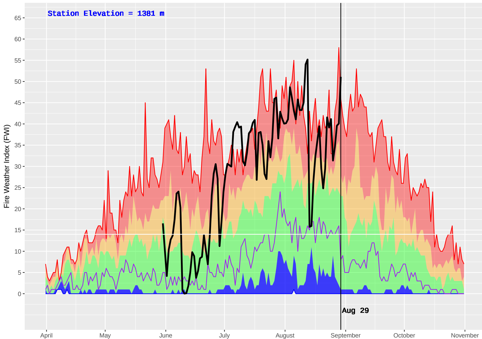
GLIMPSE (291) : Historical (1978–2016) and Current (2017) Noon Fire Weather Index (FWI)
