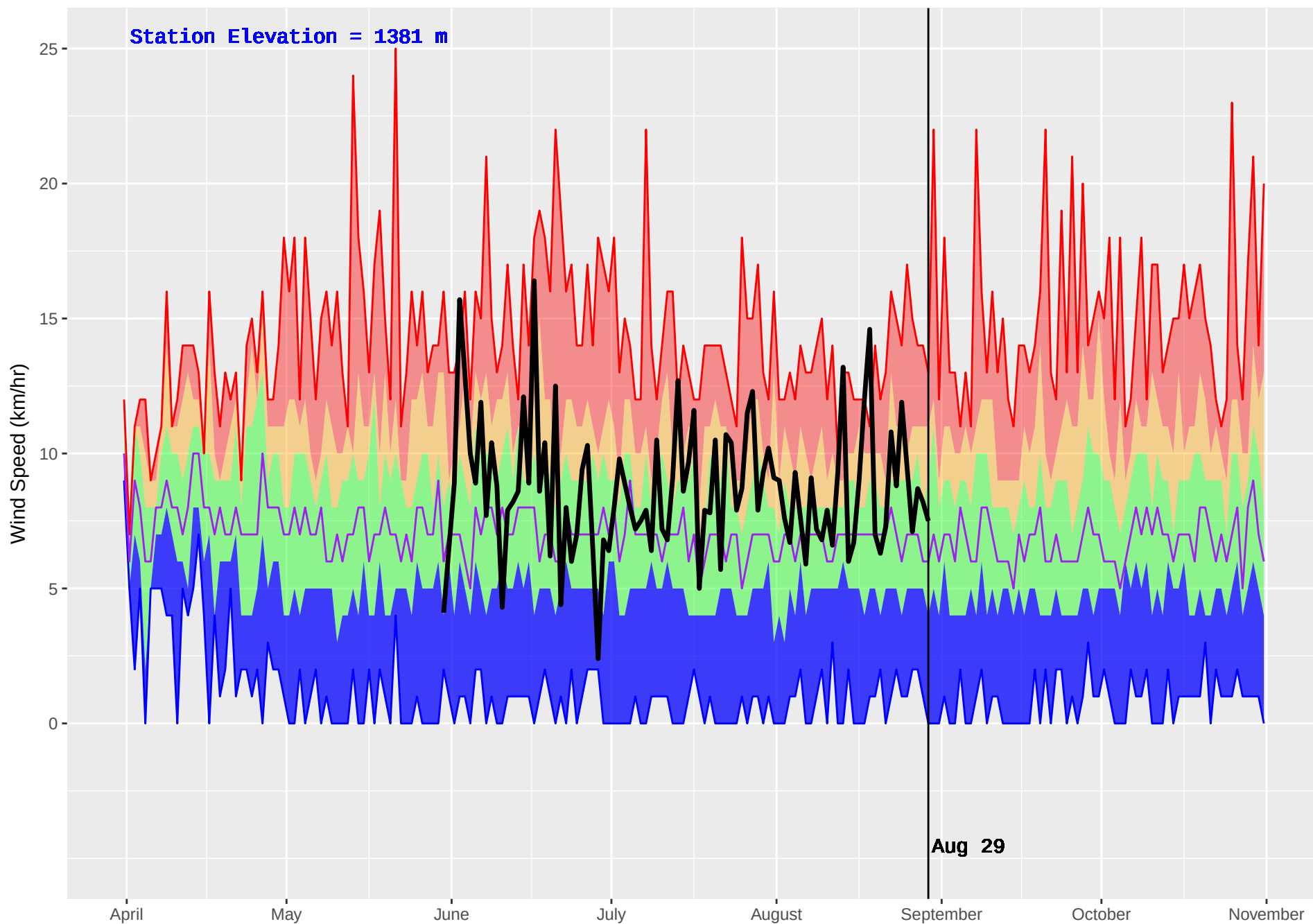
GLIMPSE (291) : Historical (1978–2016) and Current (2017) Noon Wind Speed
